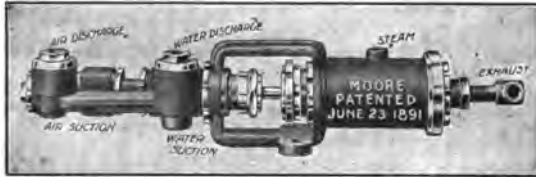
FIG. 202.—The Moore Steam Pump arranged to operate both Air and Water Supply for Steam Carriages.
